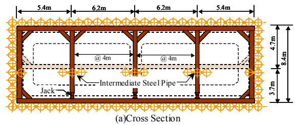
Fig. 4. Configuration of Steel Pipe Interlocking Design
