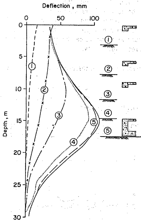
Figure 5 Wall Deflections During Excavation
