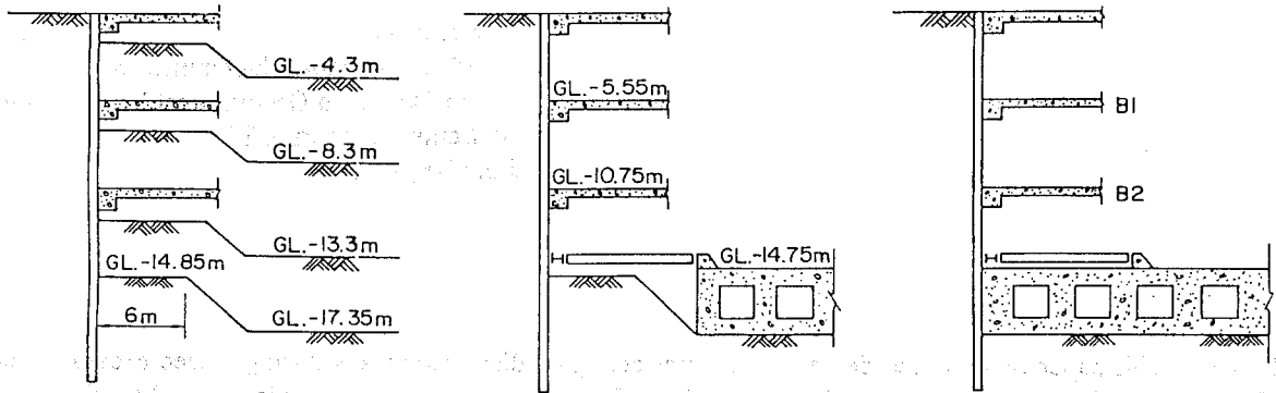
Figure 2 Sequence of Excavation
