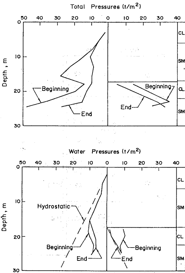
Figure 3 Distribution of Total and Water Pressures
