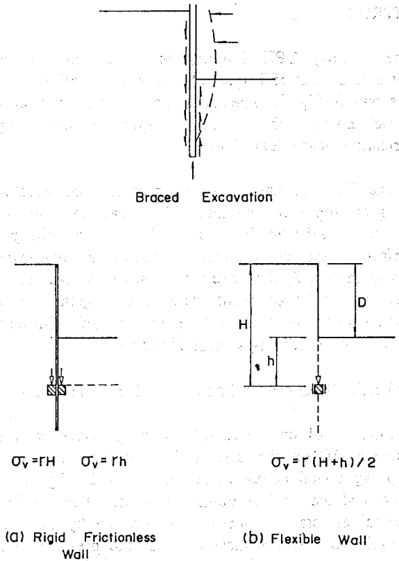
Figure 4 Vertical Earth Pressures as Affected by Characteristics of Wall
