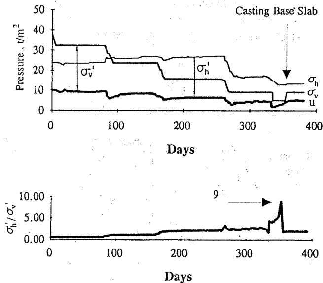
Figure 10 Passive Pressure at a Depth of 20m
