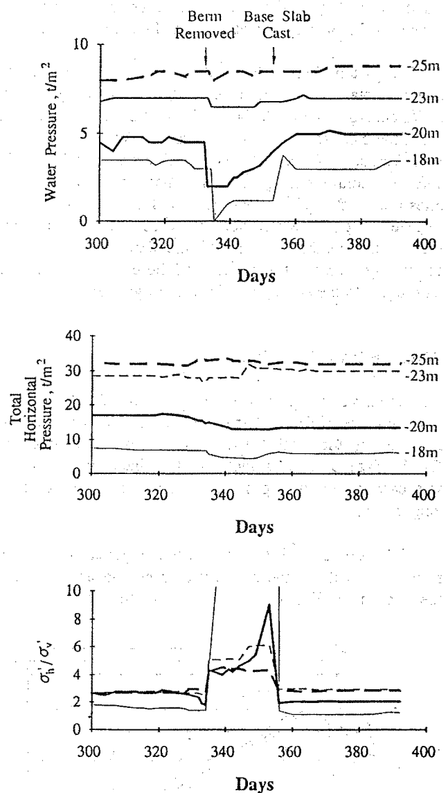
Figure 11 Results for All Cells on the Passive Side
