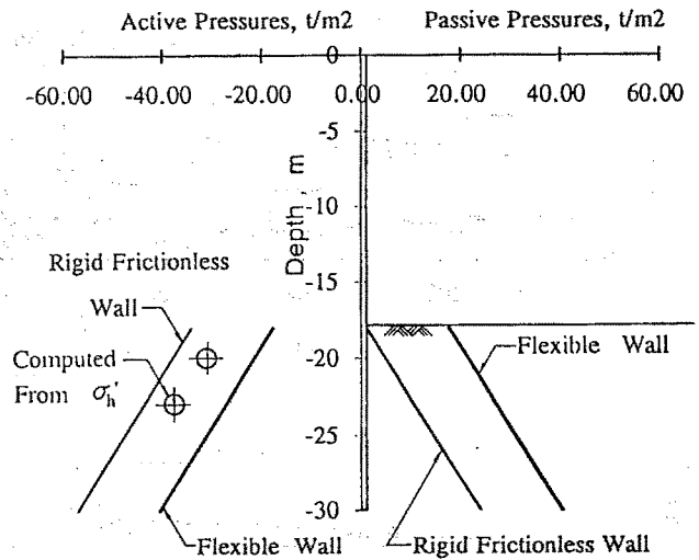
Figure 9 Computed Vertical Pressures
