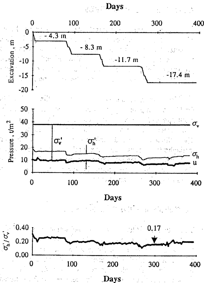
Figure 6 Active Pressures at a Depth of 20m
