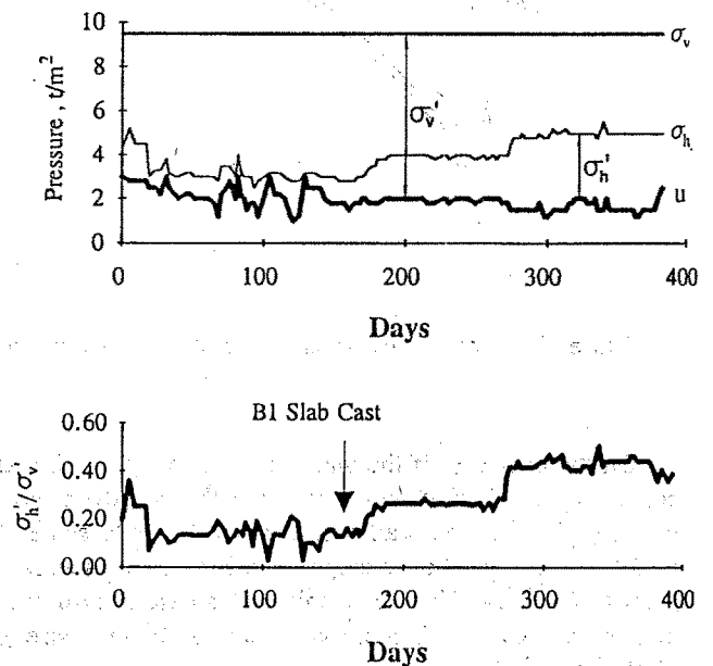
Figure 7 Active Pressures at a Depth of 5m
